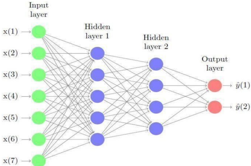
Fig 5.4 CNN classification
