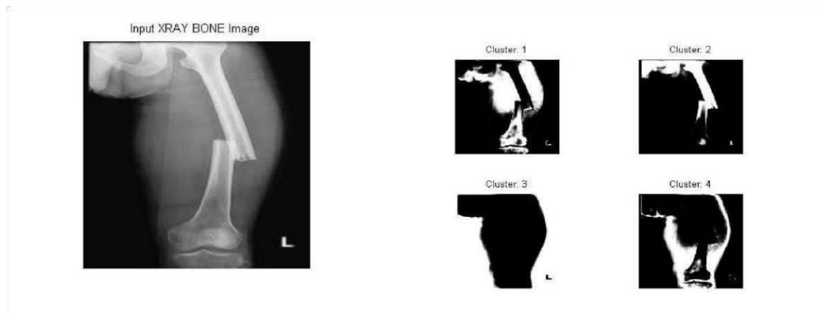
Fig 6.3 Filtered Image
