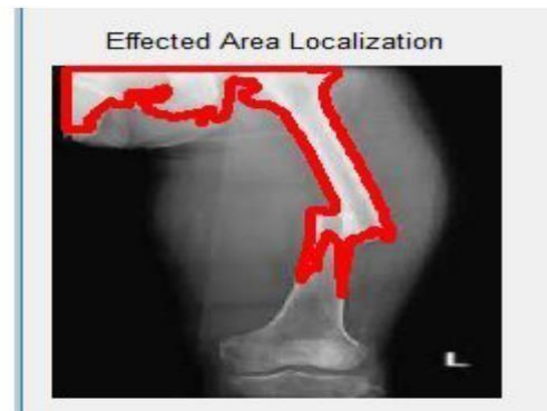
Fig6.6 Effected Image
