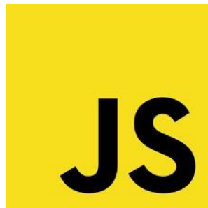
Fig 3.4 JAVASCRIPT LOGO
