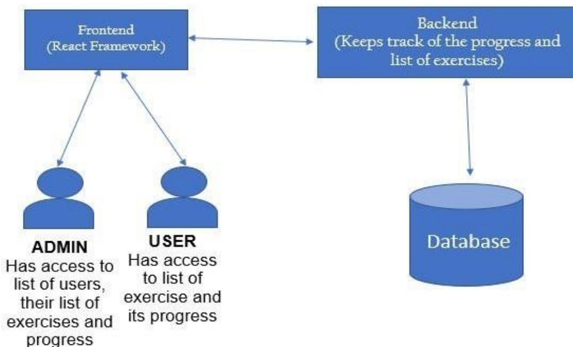
Fig 4.1 Architecture Diagram
