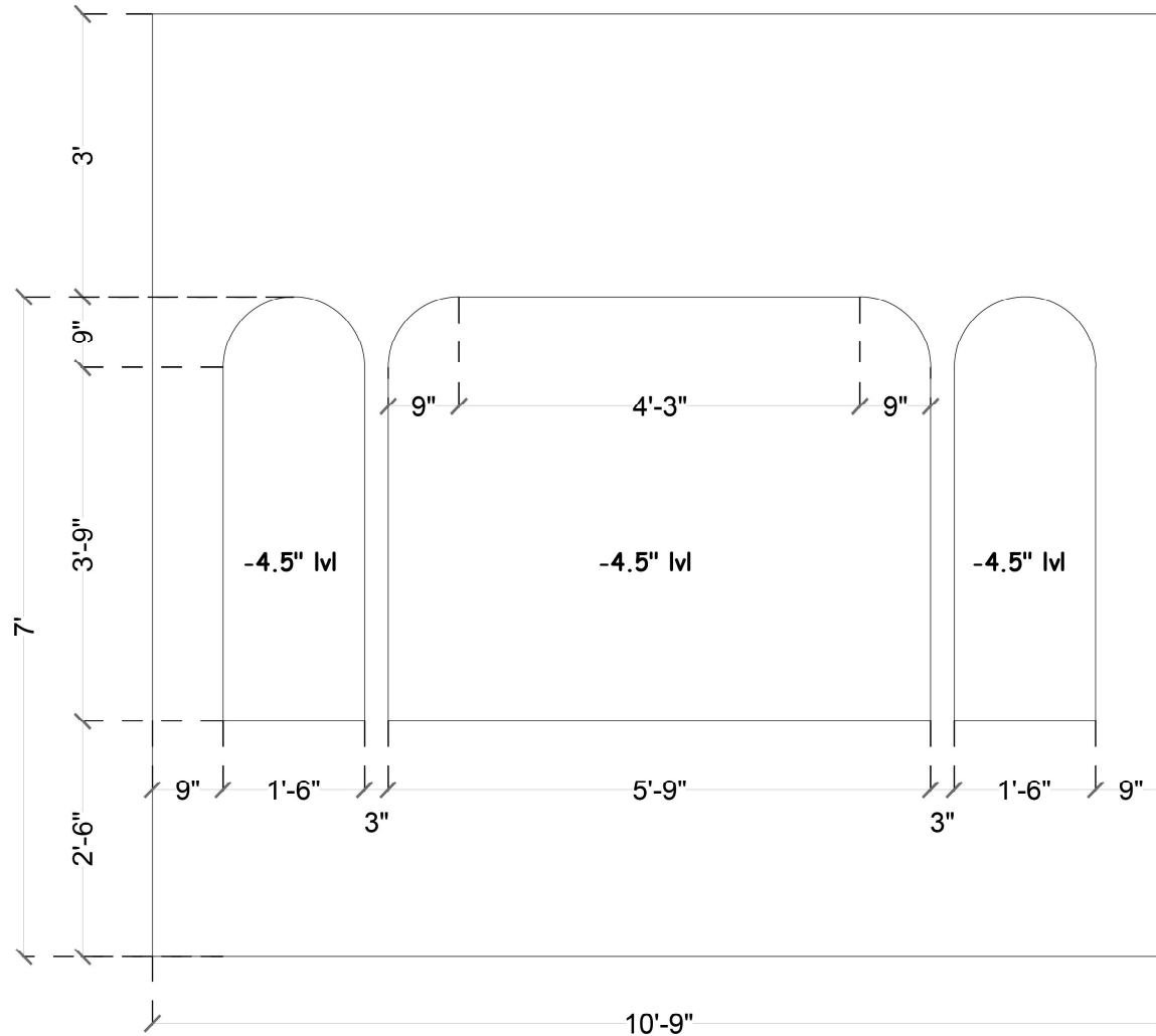
SOFA WALL ELEVATION
