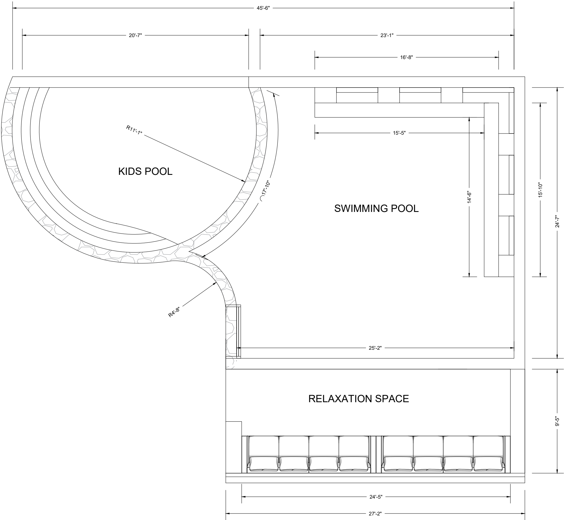
CLUBHOUSE : SWIMMING POOL WORKING DRAWING
