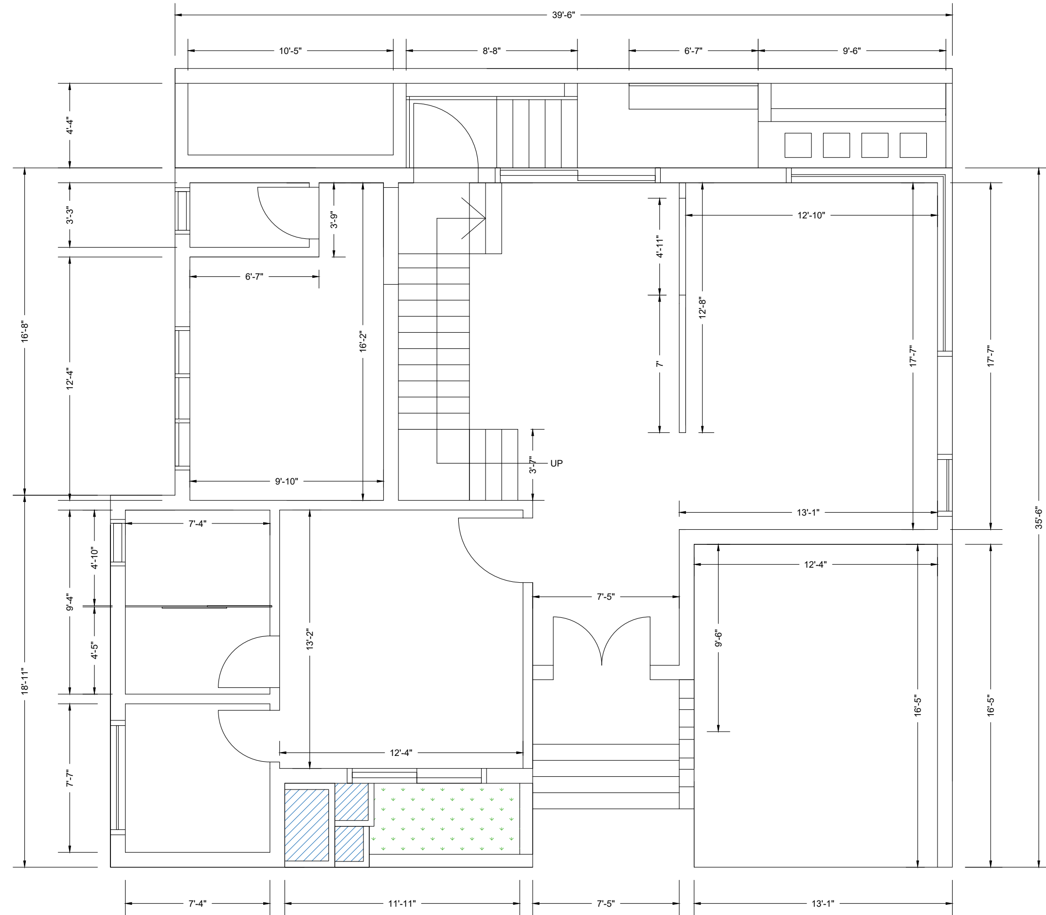
VILLA B : GROUND FLOOR WORKING DIAGRAM
