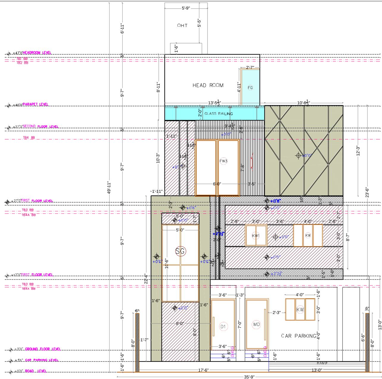
1 RO – NORTH DIRECTION ELEVATION
