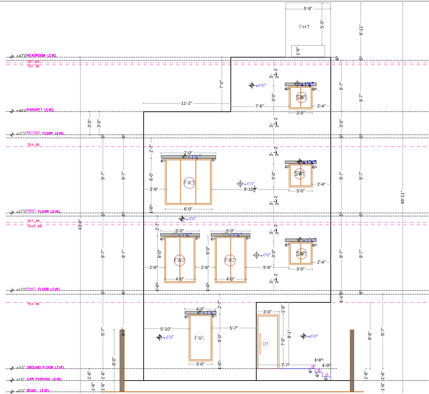
3 R0 - S0 TH DIRECTION ELEVATION
