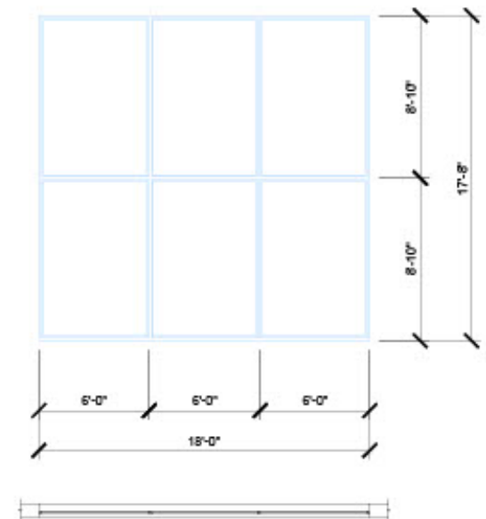
GLAZING DETAIL FOR EAST ELEVATION
