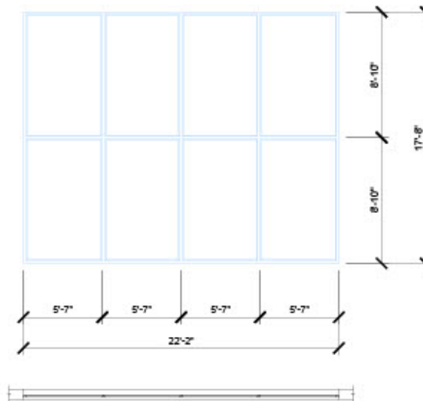
GLAZING DETAIL FOR SOUTH ELEVATION
