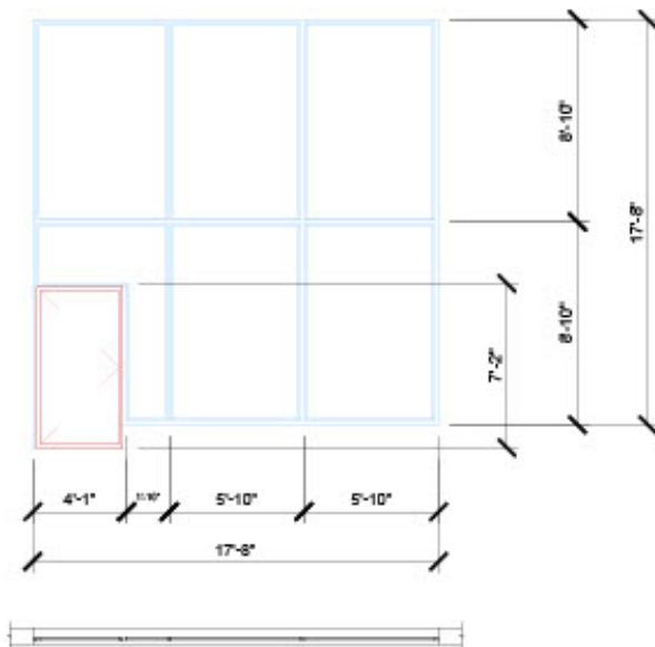
GLAZING DETAIL FOR STAIRCASE ELEVATION
