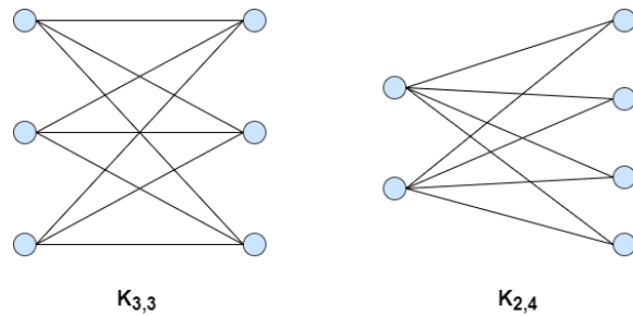
Fig 1.1 Bipartite graph
