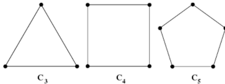
Fig 1.3 Cyclic Graphs
