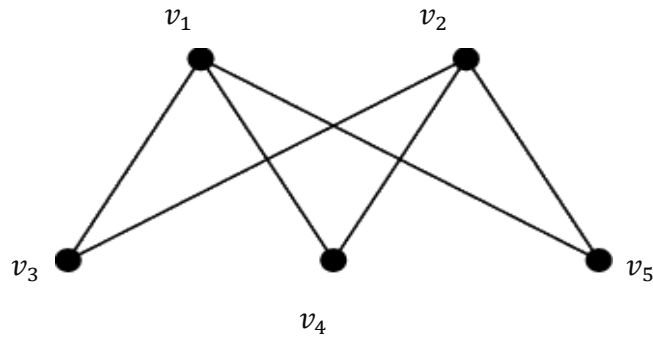
Fig 1.2 Complete bipartite graph
