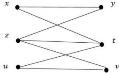
Fig 4.1 Example graph G (bipartite)
