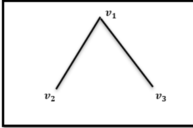
Fig 5.1 Graph G with 3 vertices
