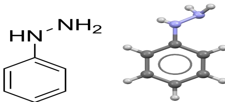
Fig 1.8: Phenyl hydrazine
