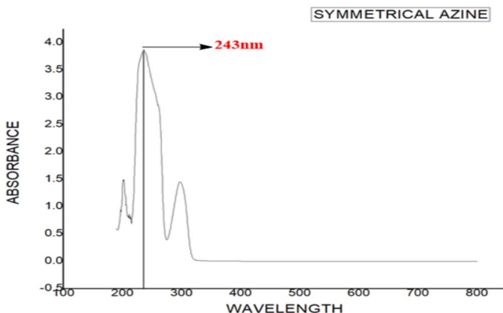
Fig 5.1: Spectrum of UV
