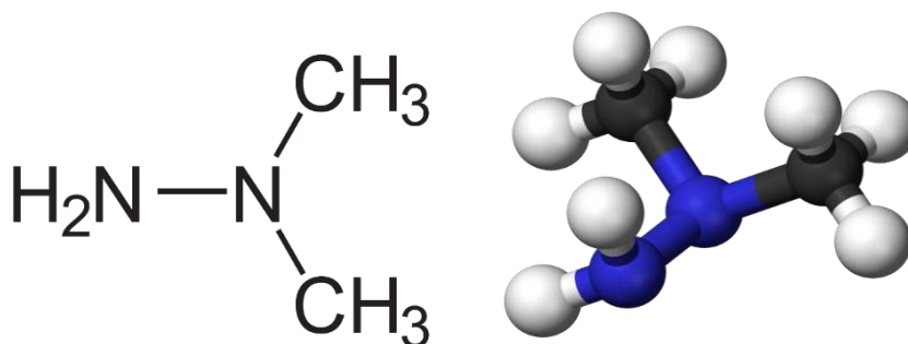
Fig 1.7 : 1,1-Dimethyl hydrazine
