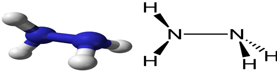
Fig:1.5: Hydrazine
