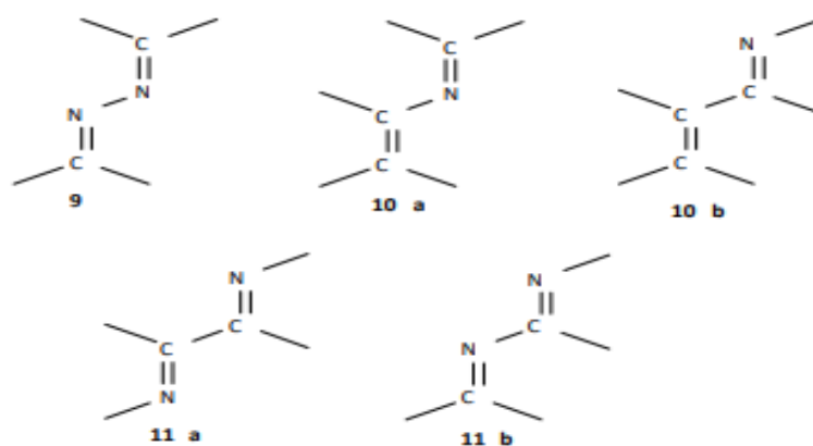
Fig:1.4:azines 9, enimes 10a and 10b, and 1,2-diimines 11a and 11b
