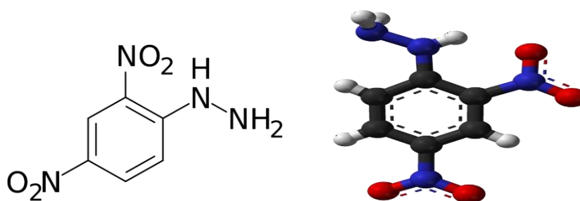
Fig 1.9: 2,4-Dinitrophenylhydrazine (2,4-DNPH)
