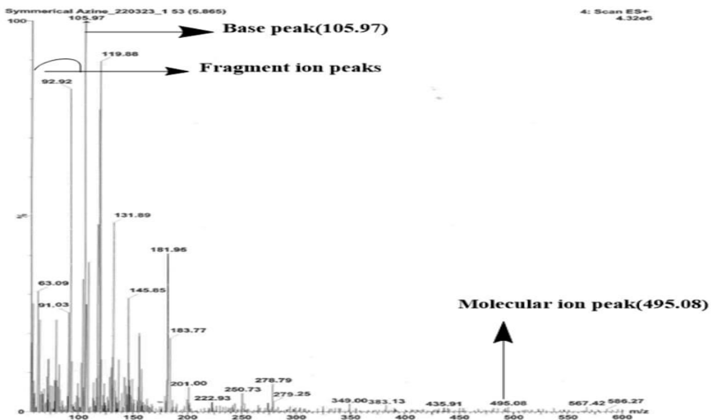
Fig 5.7: Spectrum of mass
