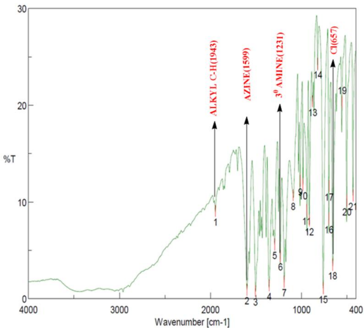
Fig 5.2: FTIR Analysis Of Azine
