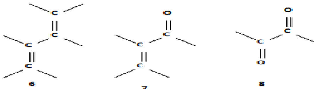
Fig:1.3: 1,3-dienes [6], enones [7], and 1,2-diones [8]
