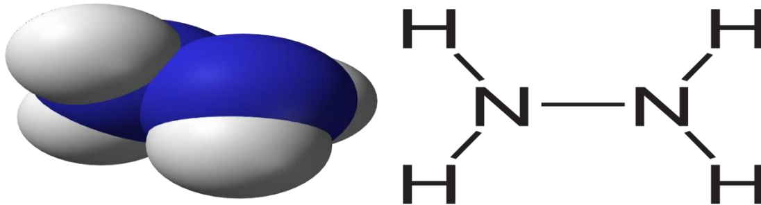
Fig:1.6: Hydrazine
