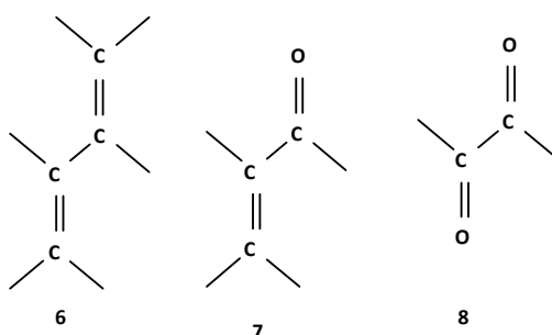
Fig:1.3: 1,3-dienes [6], enones [7], and 1,2-diones [8]
