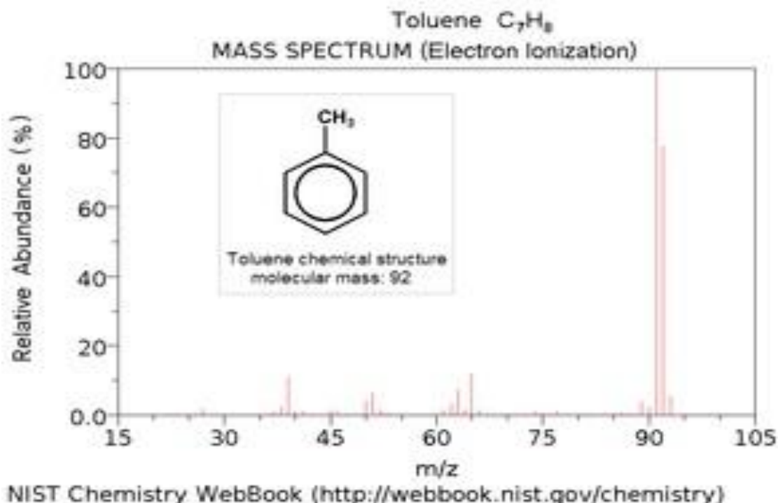
Fig 4.4: Mass spectrum
