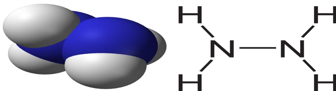
Fig:1.6: Hydrazine
