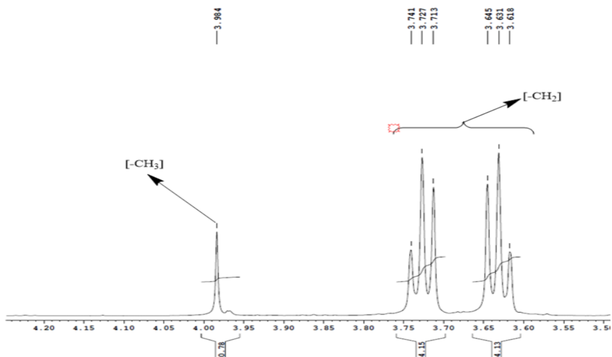
Fig 5.6: Spectrum of ^1\text{H} NMR
