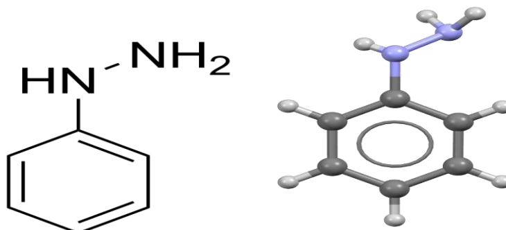
Fig 1.8: Phenyl hydrazine
