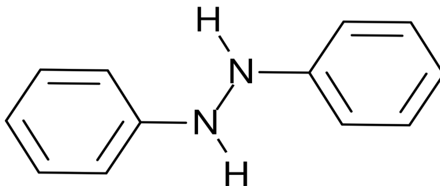
Fig 1.10: 1,2-Diphenyl hydrazine
