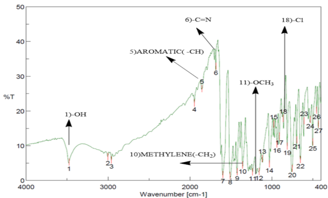
Fig 5.2: FTIR Analysis Of Unsymmetrical Azine
