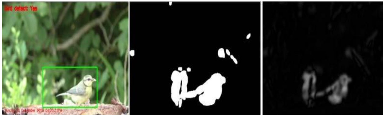
Figure 5. Shows the code detecting birds using video input.
