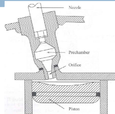
Fig. 12.21 Precombustion Chamber
