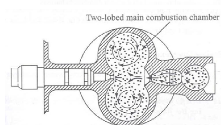
Fig. 12.22 Lanova Air-Cell Combustion Chamber
