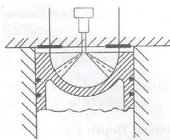
(b) Hemispherical chamber
