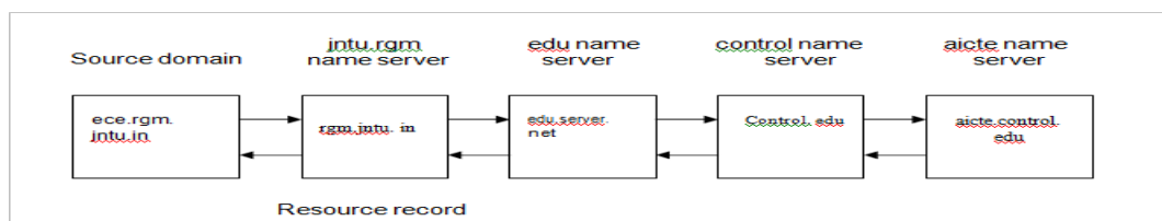
Figure 5.3. Domain Name System Example
