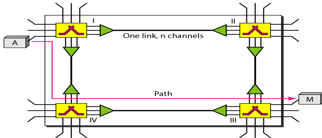
Figure 1.28 circuit-switched network
