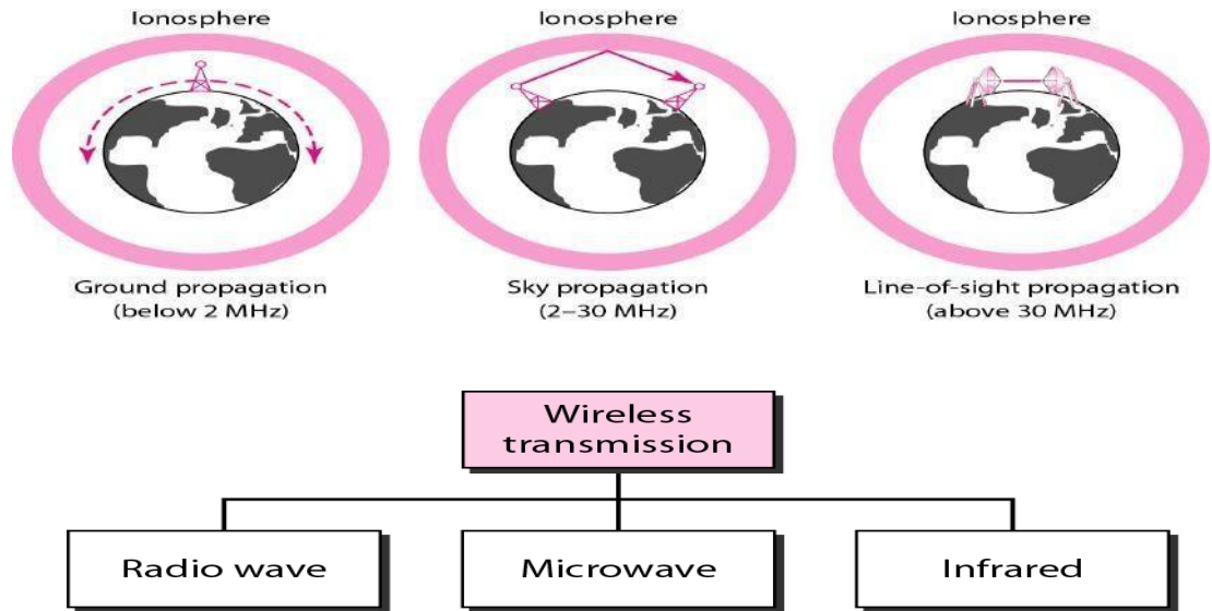
Figure 1.23 Types of Unguided media
