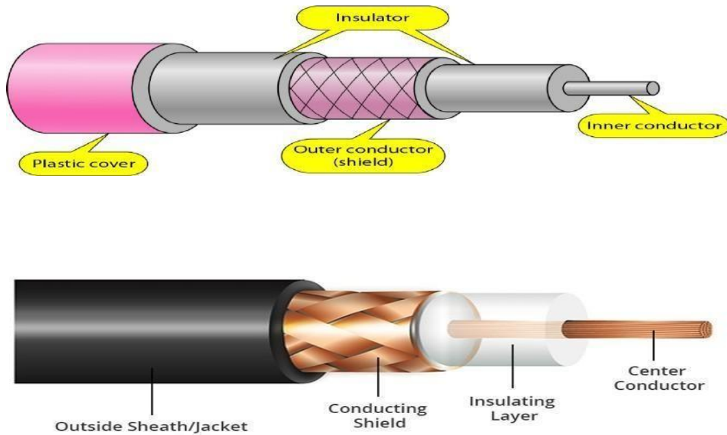
Figure 1.17 Coaxial cable
