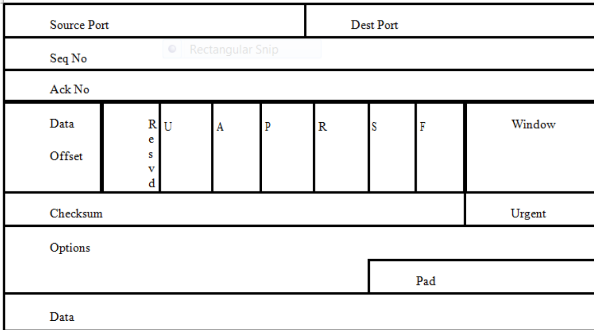
Fig3.3:TCP Header
