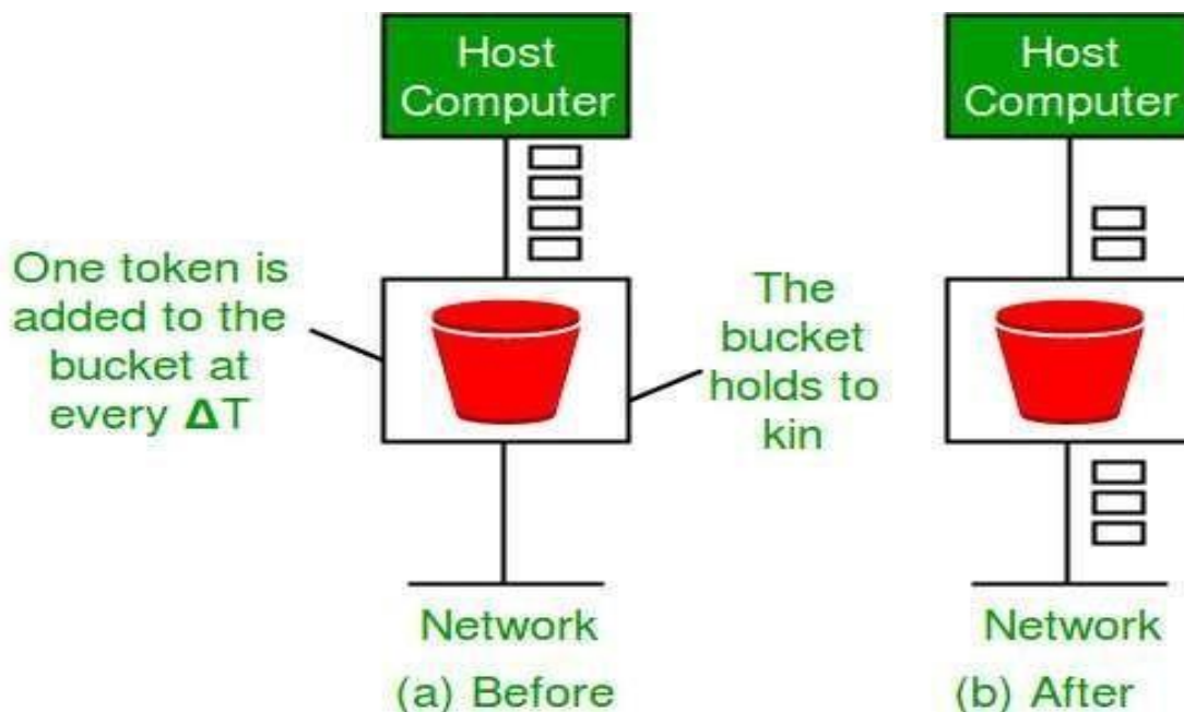
Fig3.6: Token Bucket Algorithm
