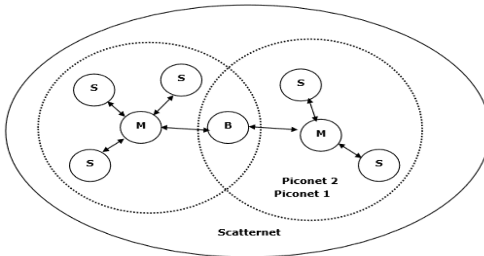
Figure: Piconets and Scatternets
