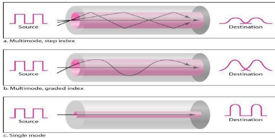
Figure 1.21 Types of Modes
