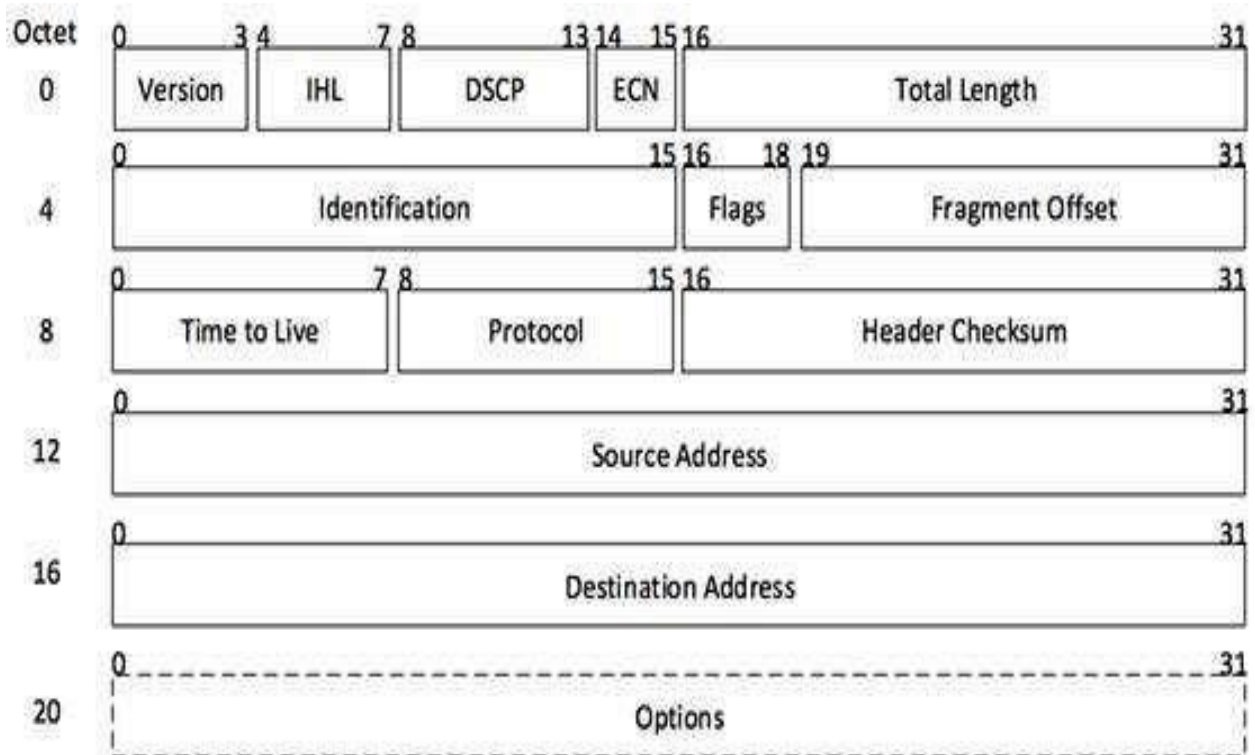
[Image: IP Header]
