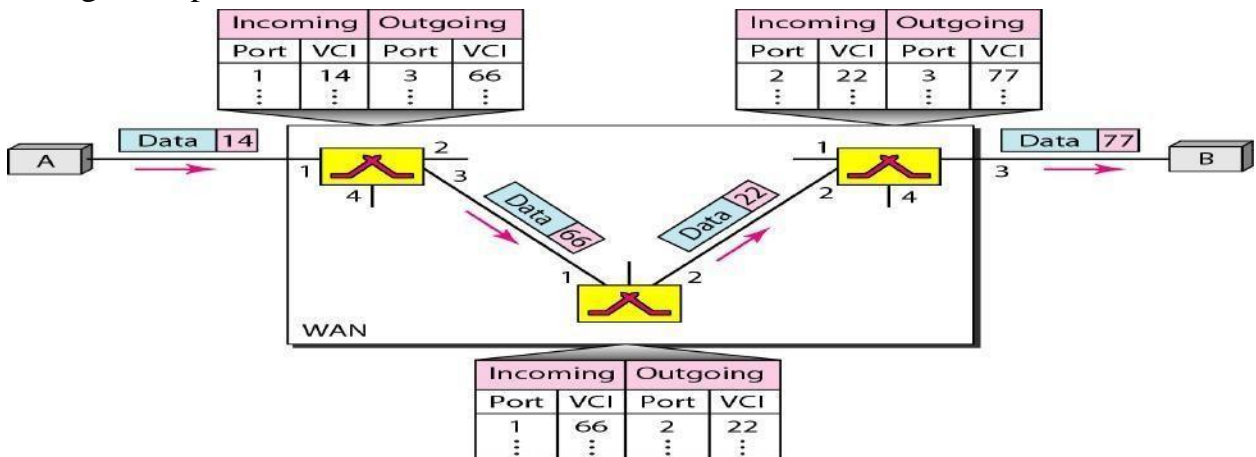
Figure 1.34 VCI changes during the trip
