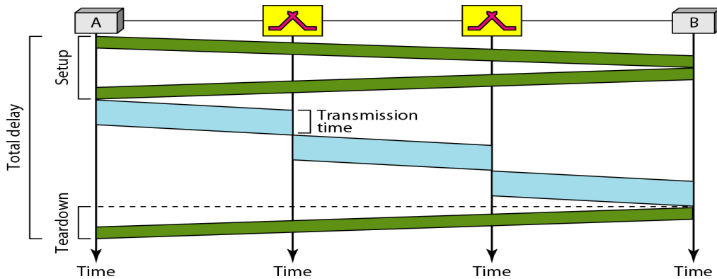
Figure 1.37 virtual-circuit network delay
