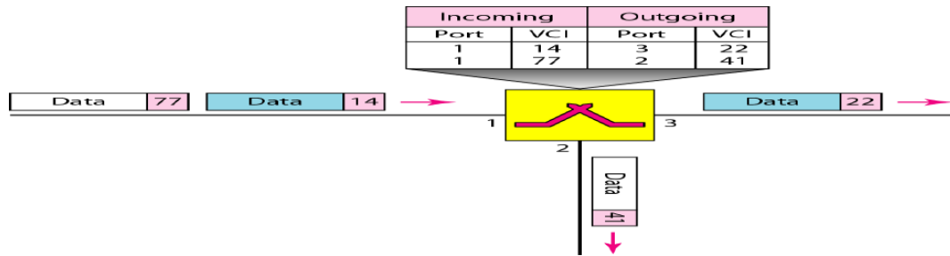
Figure 1.33 Data Transfer Phase
