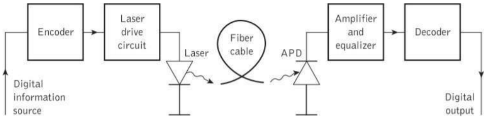
Figure 3: A digital optical fiber link using a semiconductor laser source and an avalanche photodiode (APD) detector.
