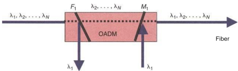
Figure 5.8 The optical add—drop multiplexer is a DWDM function.
