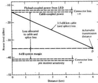
Figure 4.17 Link Power Budget Graph
