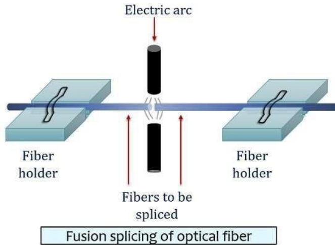
Figure 4.13 Fusion Splicing of Optical Fiber
