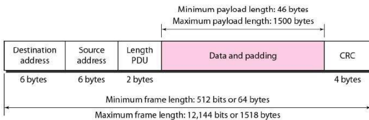
Figure 5.3 Minimum and maximum lengths
