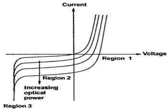
Figure. 3.7 V-I Characteristics of Photodiode
