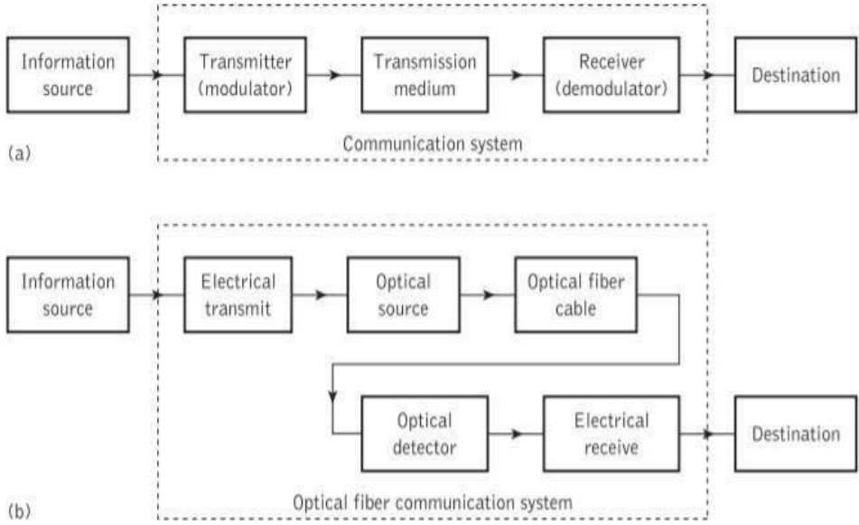
Figure2: (a) The general communications system. (b) The optical fiber communication system
