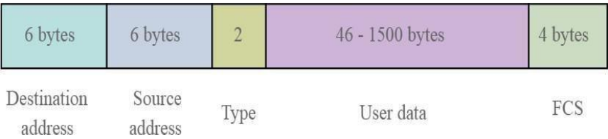
Figure 5.4 Basic Ethernet layer 2 frame format
