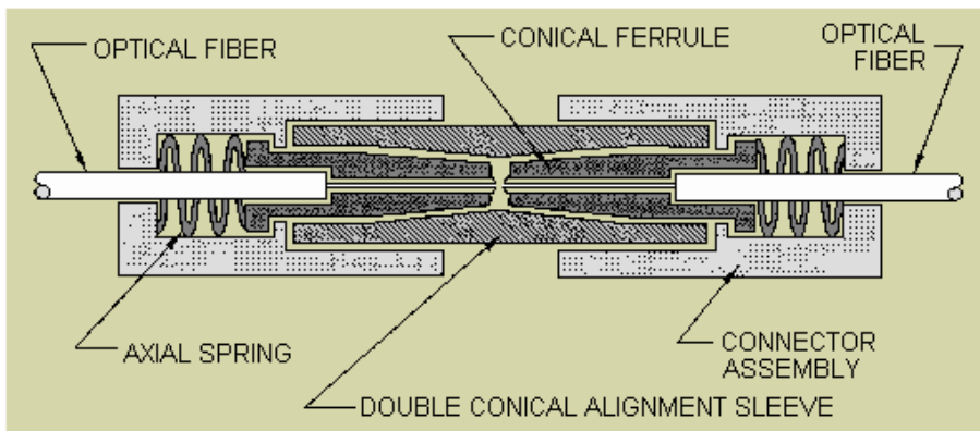
Figure 4.12 Biconical Connector
