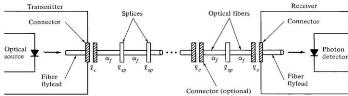
Figure 4.16 Link Power Budget
