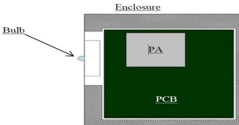
Fig 5.11: Block Diagram of Li-Fi sub-assemblies.
