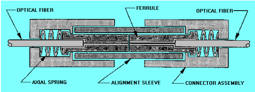
Figure 4.10 Basic Ferrule Connectors
