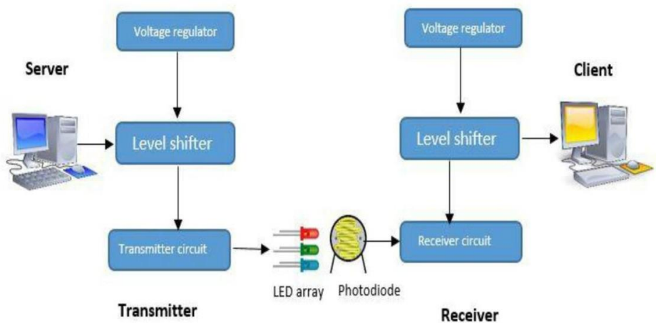
Fig 5.13: Construction of Li-Fi System
