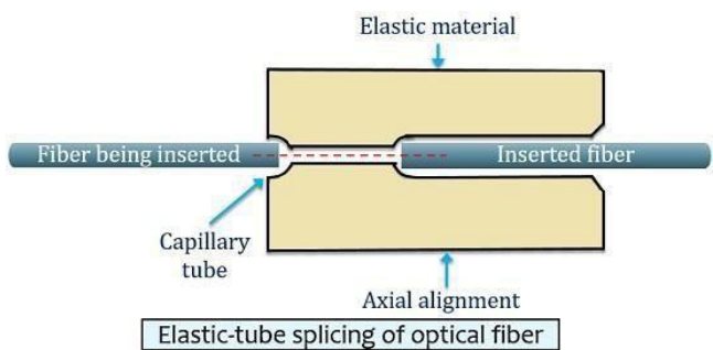
Figure 4.14 Elastic-Tube Splicing of Optical Fiber
