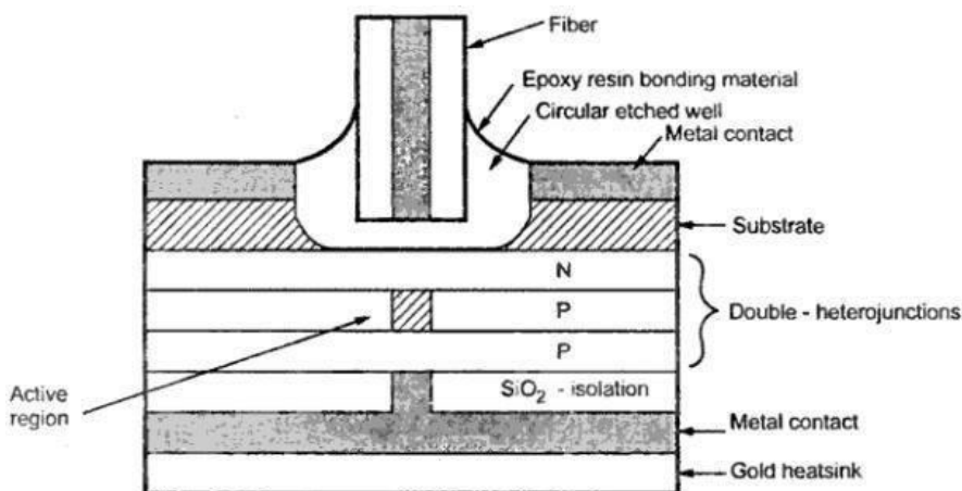
Figure 3.1 Cross section of surface emitting LED
