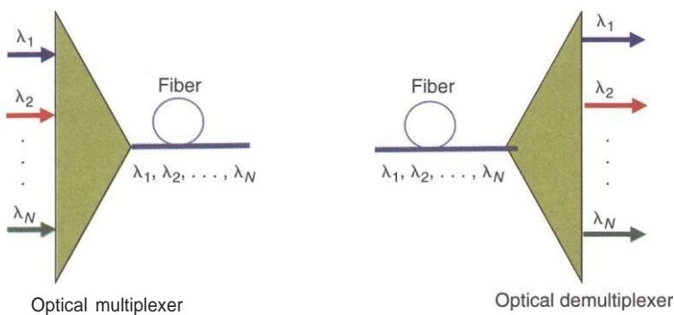
Figure 5.7 The main function of an optical multiplexer is to couple two or more wavelengths into the same fiber. The reverse takes place at a demultiplexer.
