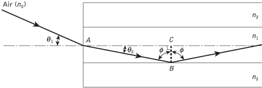
Figure 8: The ray path for a meridional ray launched into an optical fiber in air at an input angle less than the acceptance angle for the fiber
