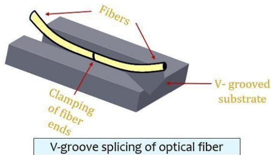
Figure 4.14 V-groove Splicing of Optical Fiber
