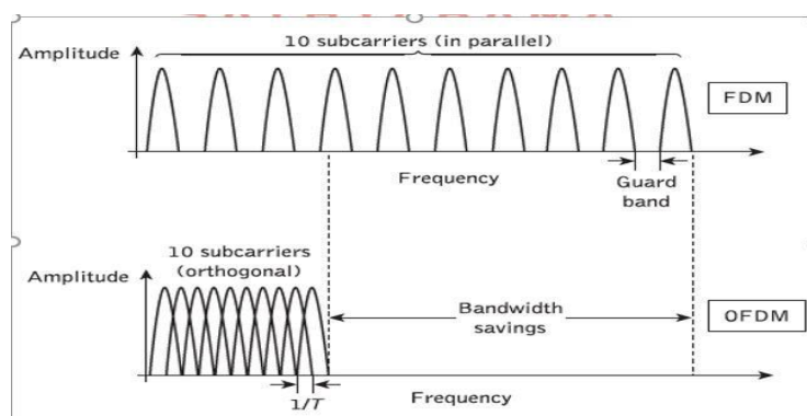
Figure 5.6 orthogonal frequency division multiplexing (OFDM) compared with conventional frequency division multiplexing(FDM)
