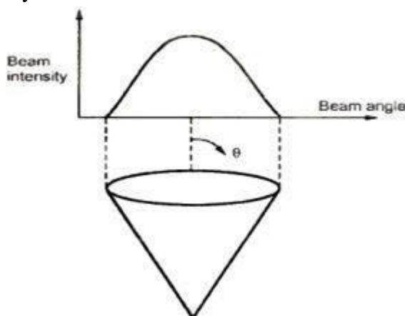
Figure. 3.2. Lambertian radiation
