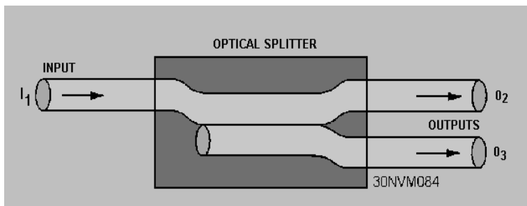
Figure 4.1 Optical Splitter
