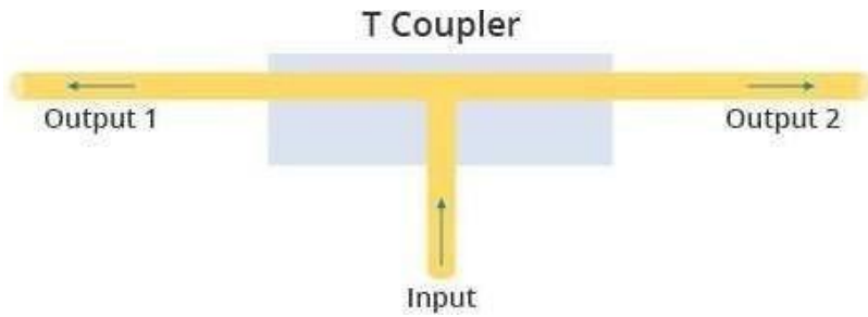
Figure 4.6 T coupler
