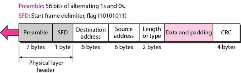
Figure 5.2 802.3 MAC frame
