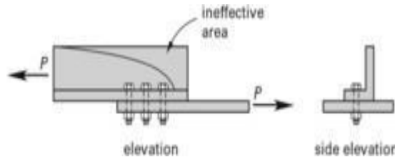
Fig.4 Shear lag effect shown on angle
