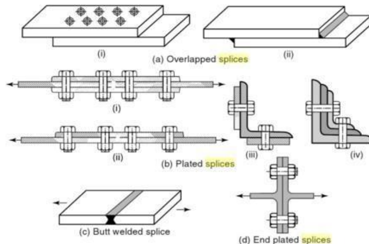
Fig.8 Typical splices in tension member
