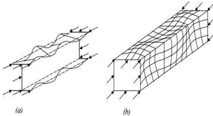
Fig. 6 Local buckling of Compression Members
