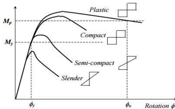
Fig. 8 Section Classification based on Moment-Rotation Characteristics
