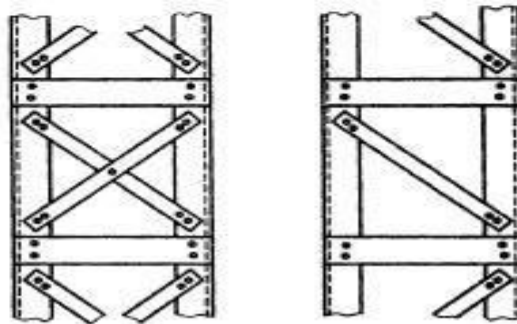
10C Double Laced and Single Laced System Combined with Cross Numbers
