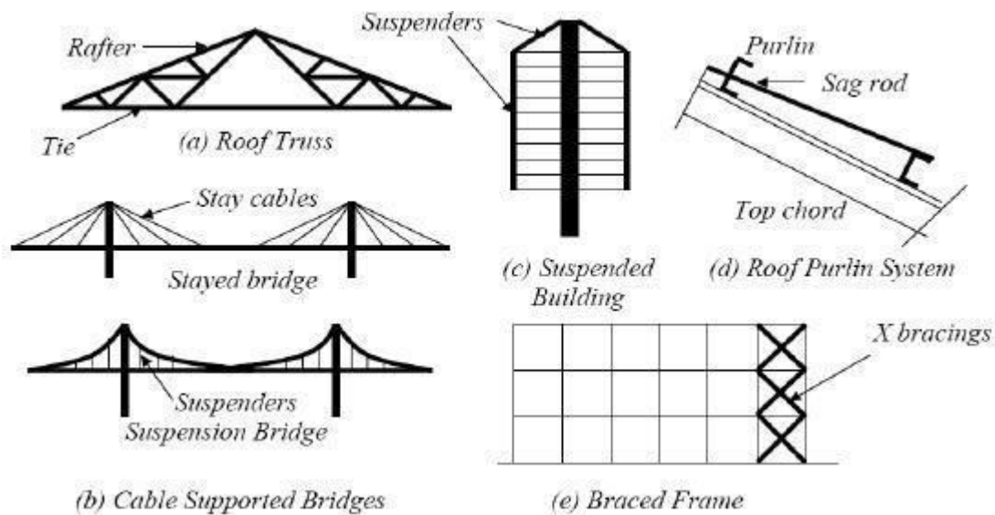
Fig. 1 Tension Members in Structures
