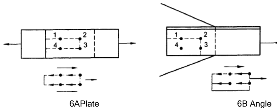
Fig.6 Block shear failure
