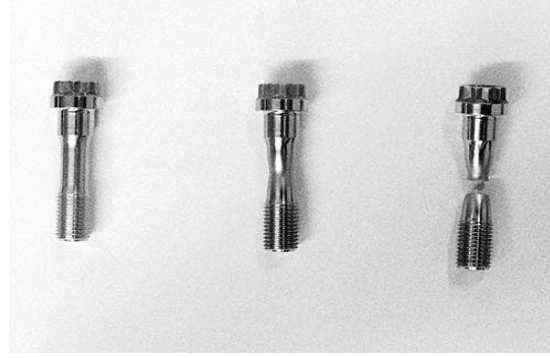
FAILURE OF BOLTS DUE TO TENSION
