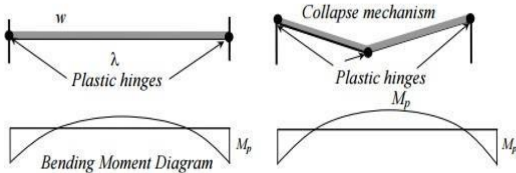
Fig. 7 Formation of a Collapse Mechanism in a Fixed Beam
