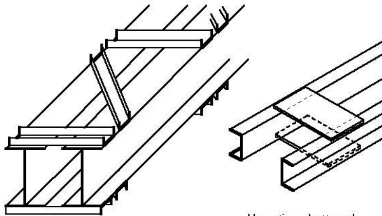
U-sections battened with flat bars
