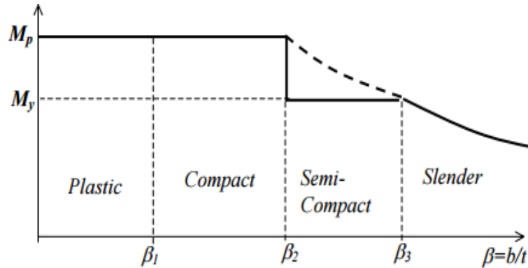
Fig 9. Section classification based on b/t ratio
