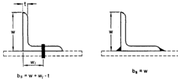
Fig. 5 Angles with single leg Connections
