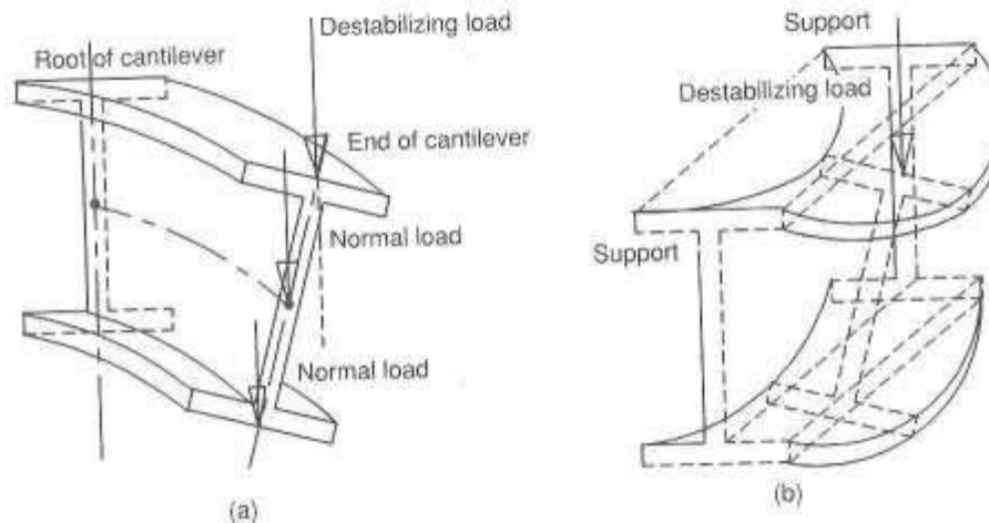
Lateral-torsional Buckling in Beams
