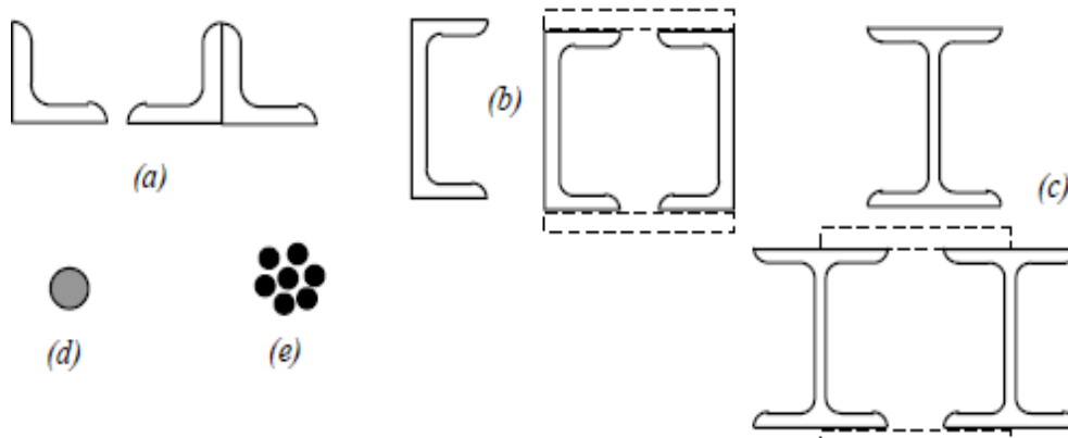
Fig. 2 Cross Sections of Tension Members
