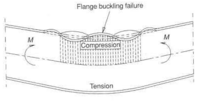
Local Flange buckling failure
