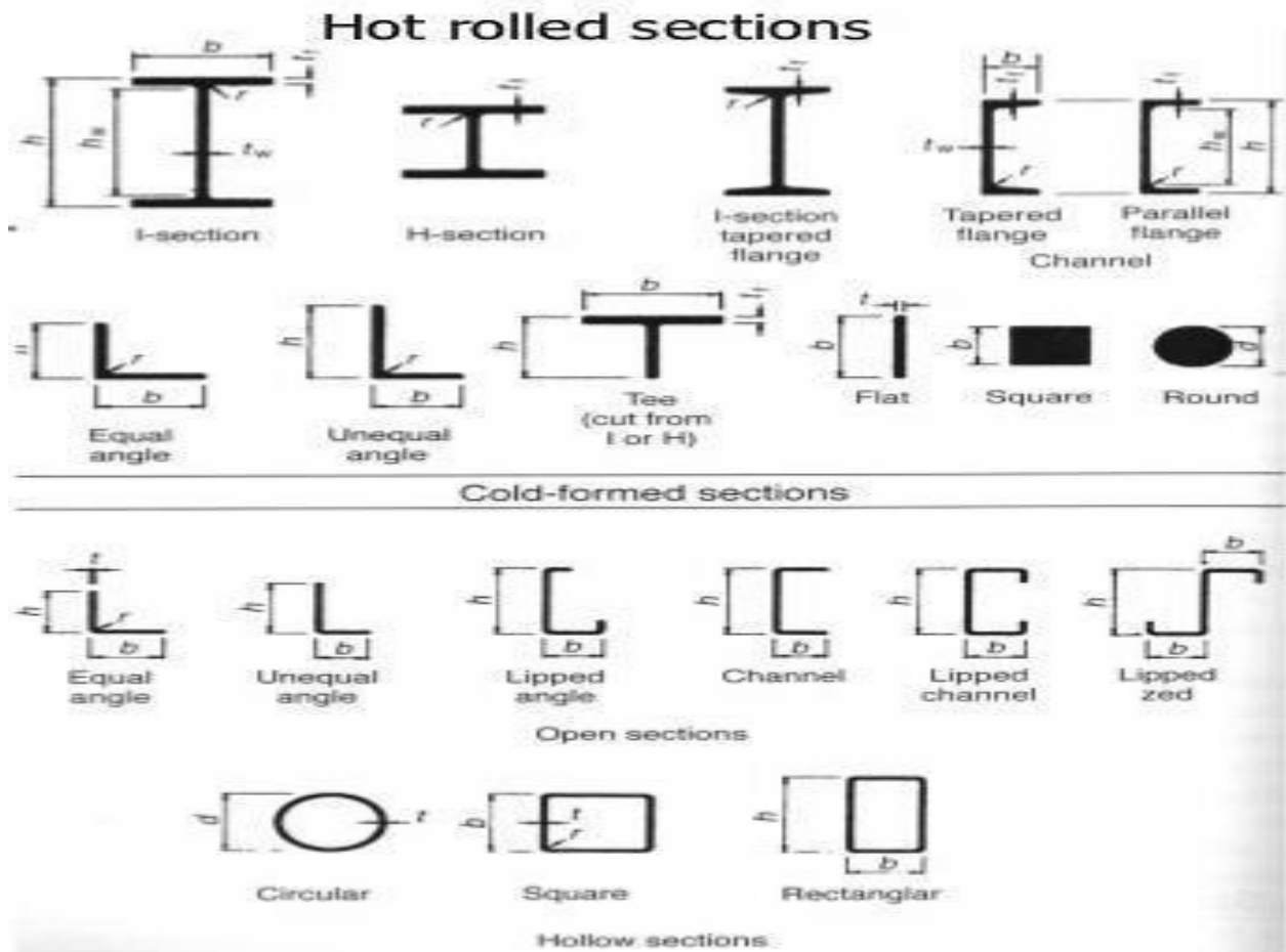
Fig 4. Hot rolled and cold formed structural sections
