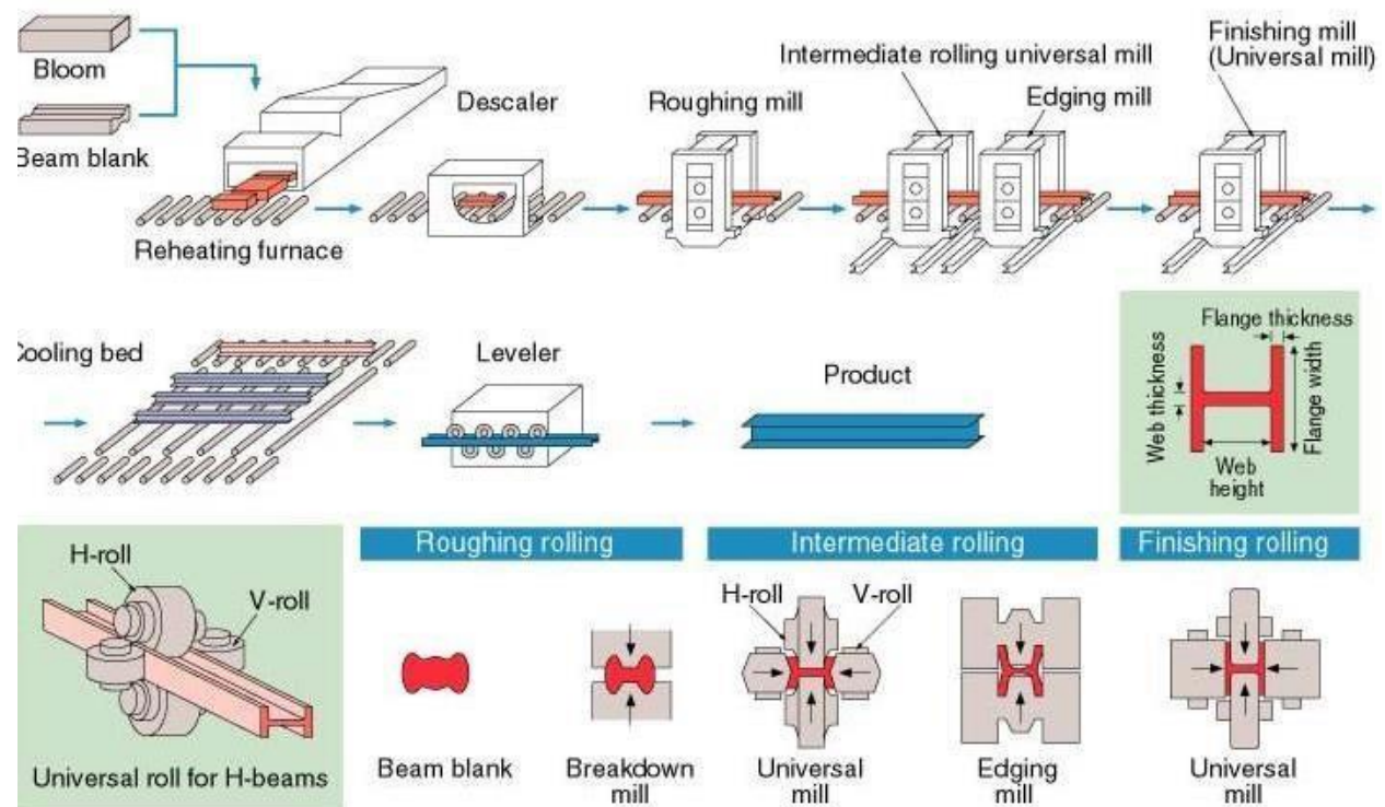
Fig 3. Manufacturing process of h beams
