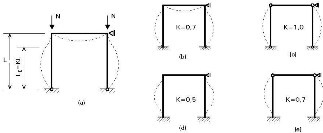
Buckling of a Column sway frame
