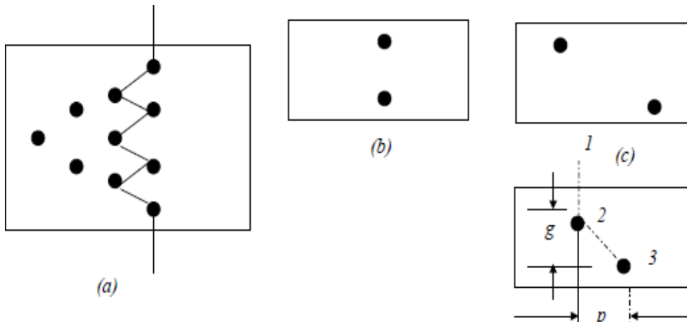
Fig. 3. Plates with Bolt Holes under Tension
