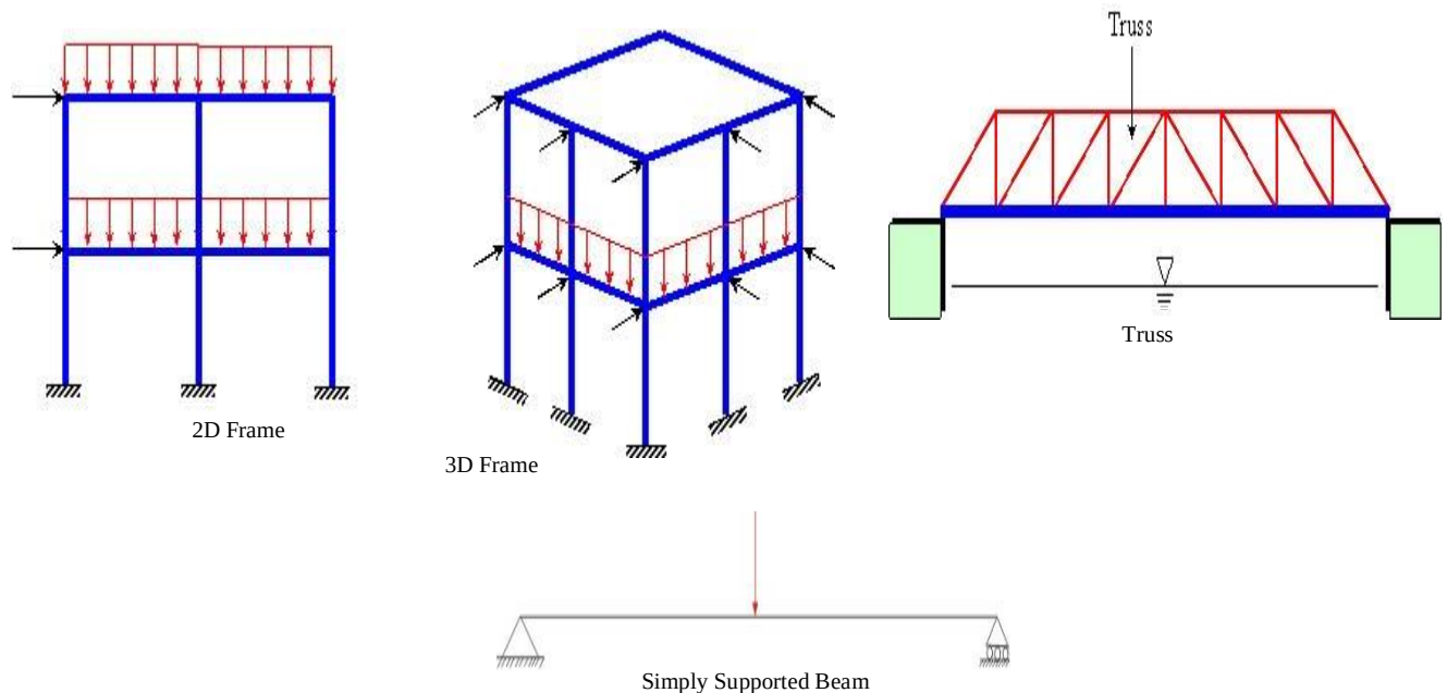
Fig 1.0 Determinate structure
