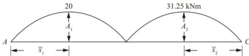
FIG. 11.1b Simple beam moment diagram
