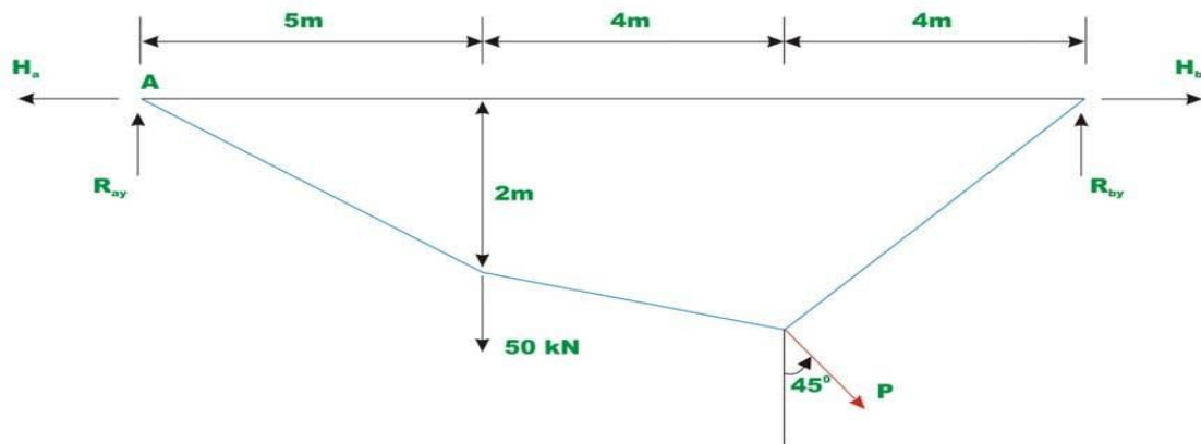
Fig. 31.6 Example 31.3
