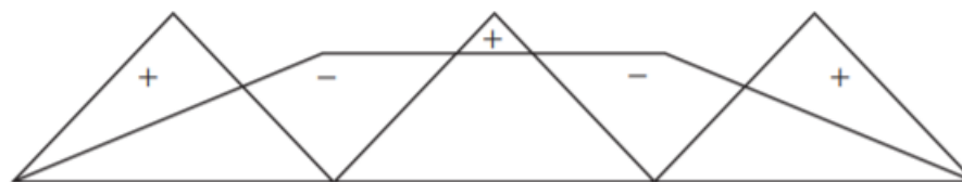
FIG. 11d Bending moment diagram
