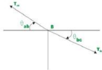
Joint B
