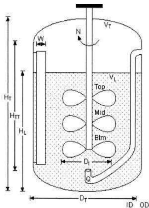
Schematic of fermentor showing nomenclature.
