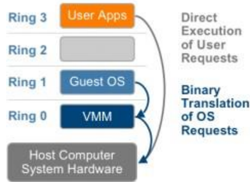
Figure 5 – The binary translation approach to x86 virtualization
