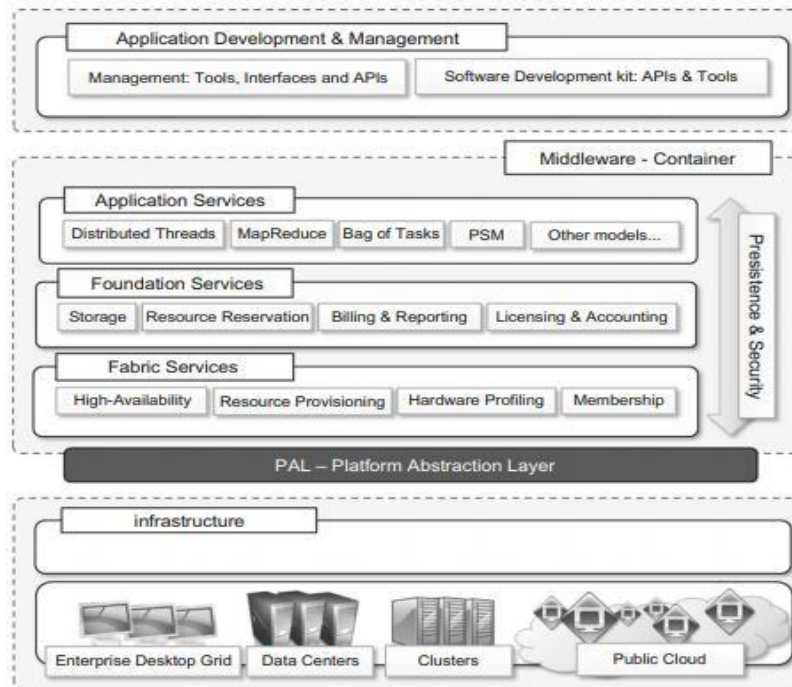
Fig 2: Architecture of Aneka
