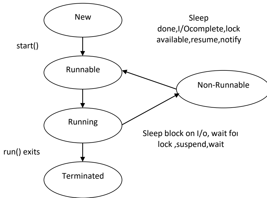
Fig. 3. 6: Thread Life Cycle
