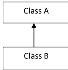
Fig. 3.1. Single Inheritance
