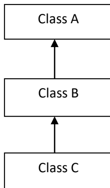
Fig. 3.2. Multiple Inheritance
