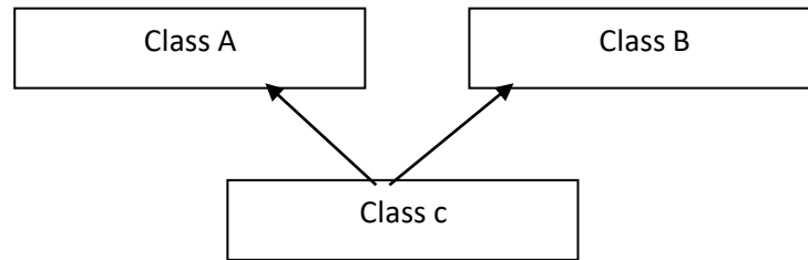
Fig. 3.4. Multiple Inheritance
