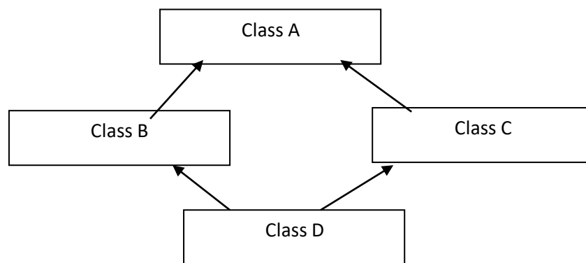
Fig. 3.5. Hybrid Inheritance
