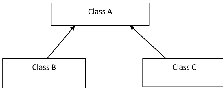
Fig. 3.3 Hierarchial Inheritance
