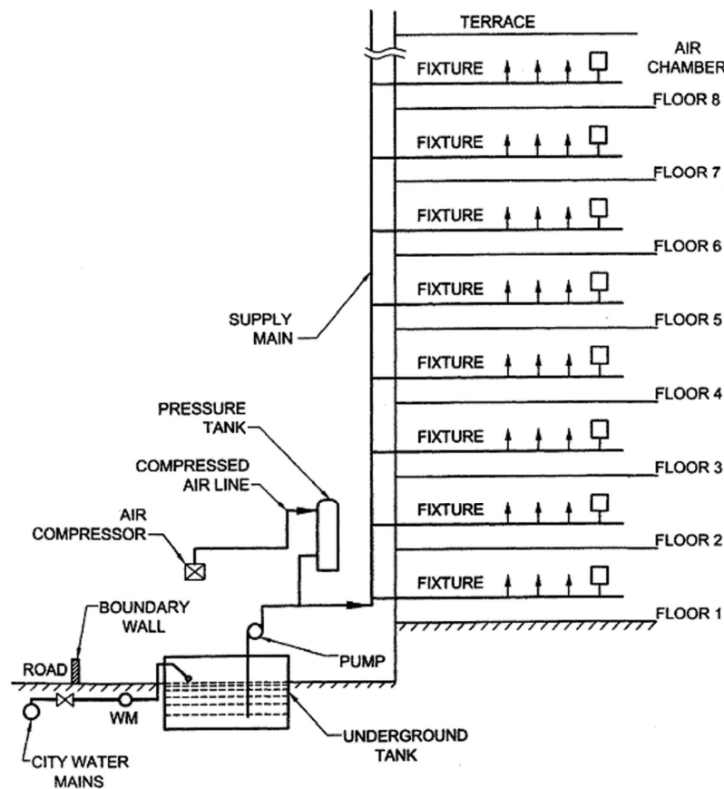
FIG. 7 HYDRO-PNEUMATIC SYSTEM
