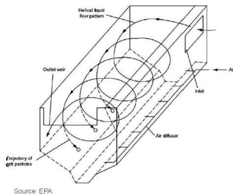
Figure 5.29 Aerated grit chamber
