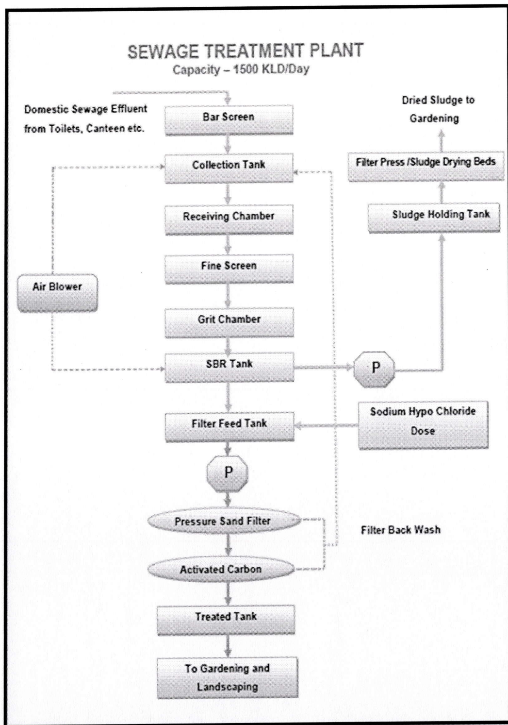
Figure 15 Sewage Treatment Plant Process Flow Diagram
