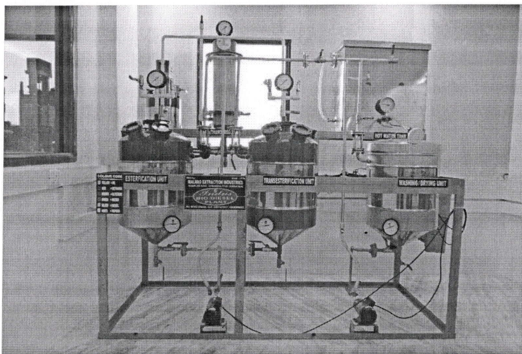
Figure 17 Pilot Scale Biodiesel Production Unit at CWM, Sathyabama
