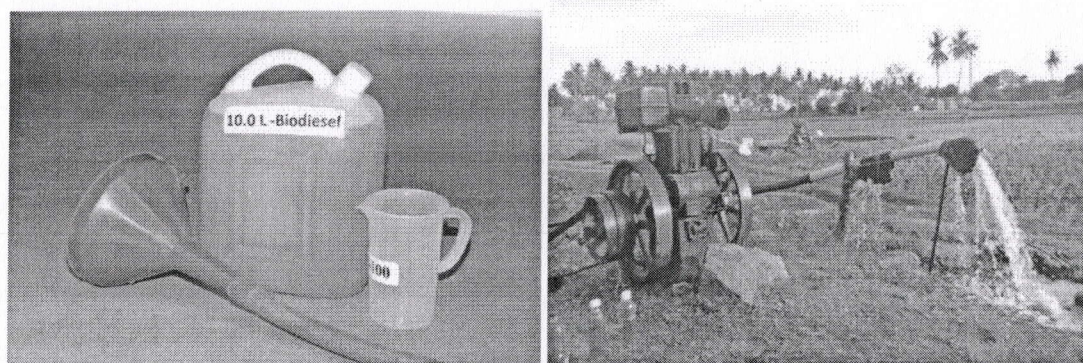
Figure 18 Biodiesel powered water pumpset
